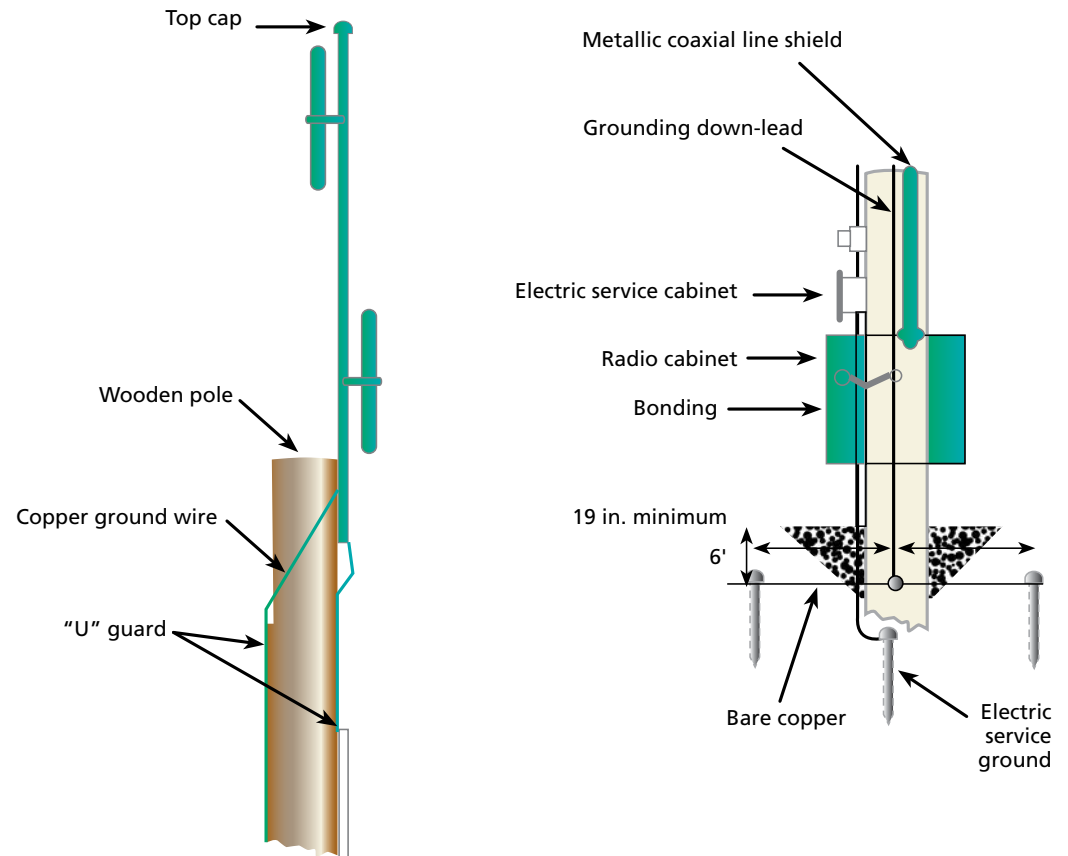
14.3: Grounding details for a wooden pole-mounted antenna
